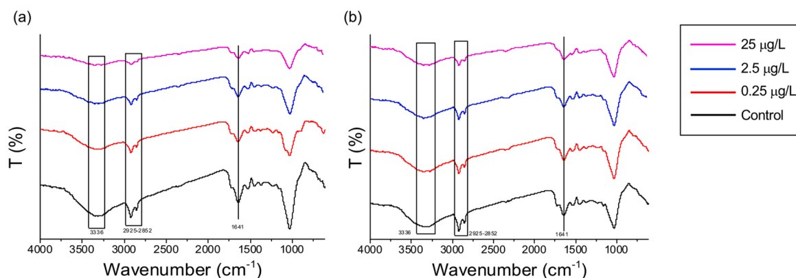
Fig. 2. Fourier-Transform Infrared (FTIR) spectroscopy of the suspensions comprising increasing concentrations (0– 25 \text{ } \mu\text{g L}^{-1} ) of small sized nanoplastics (a) and large sized nanoplastics (b) and fine particulate organic matter (FPOM) after leaf litter decomposition assay.
