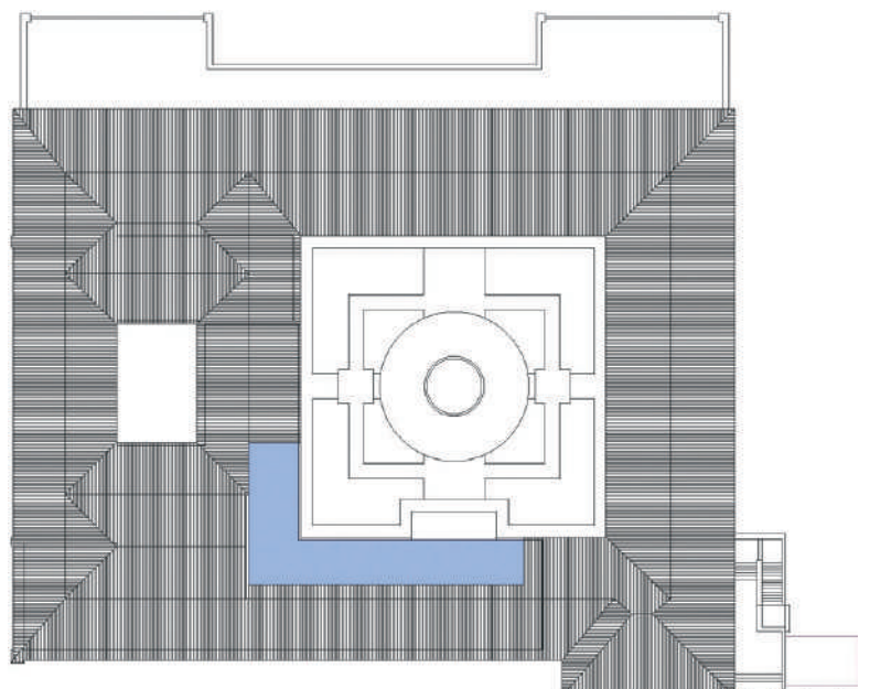
Cobertura Roof plan
