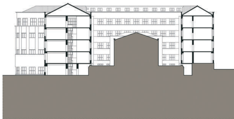
Corte sul — norte pelo pátio South-North cross section of the courtyard
