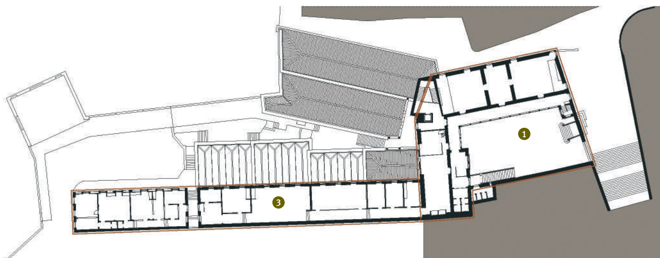
Coberturas Roof plan
